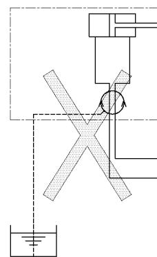
The end of drain hose is sunk in the tank of hydraulic unit.
