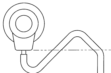
Drain hose is hanged up from the bottom line of distributor.
