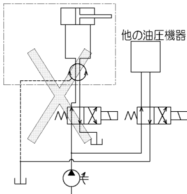
The hydraulic circuit of another actuator is connected to the drain hose.
